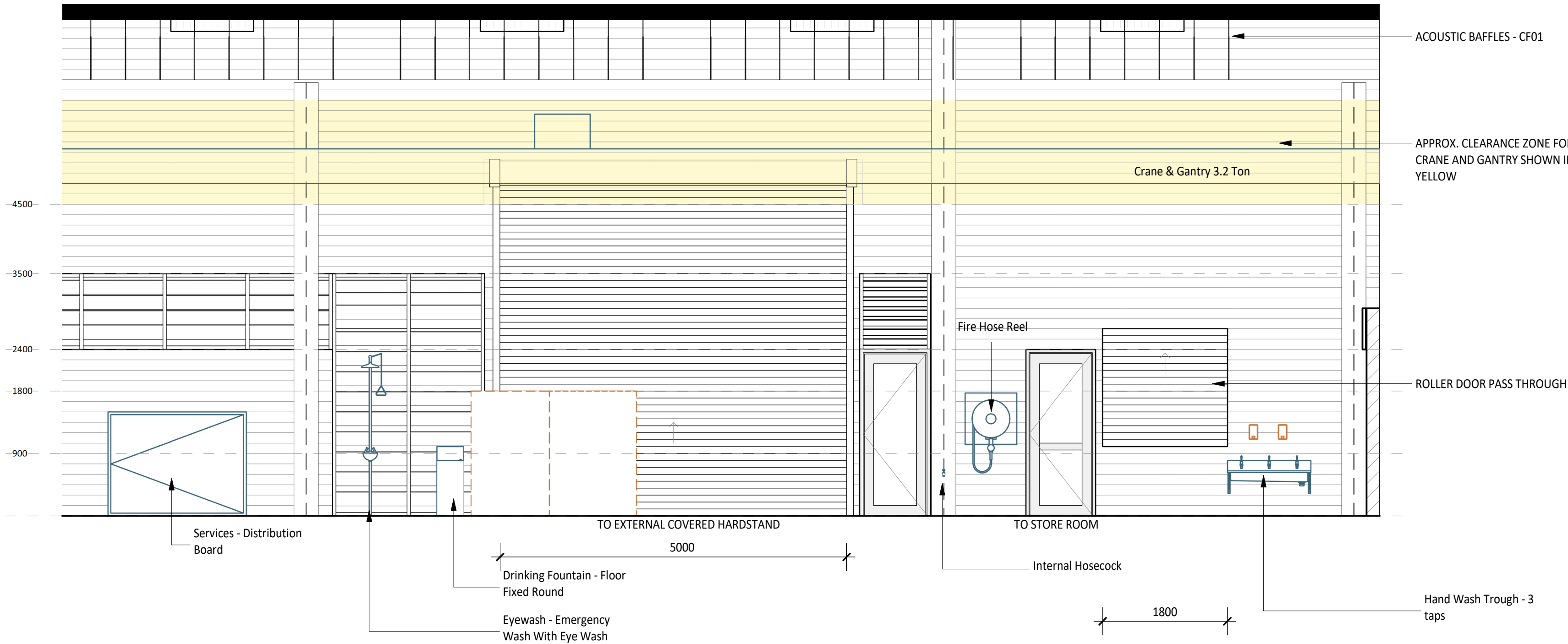
1 60-011 ELEVATION DETAIL 1 : 50
