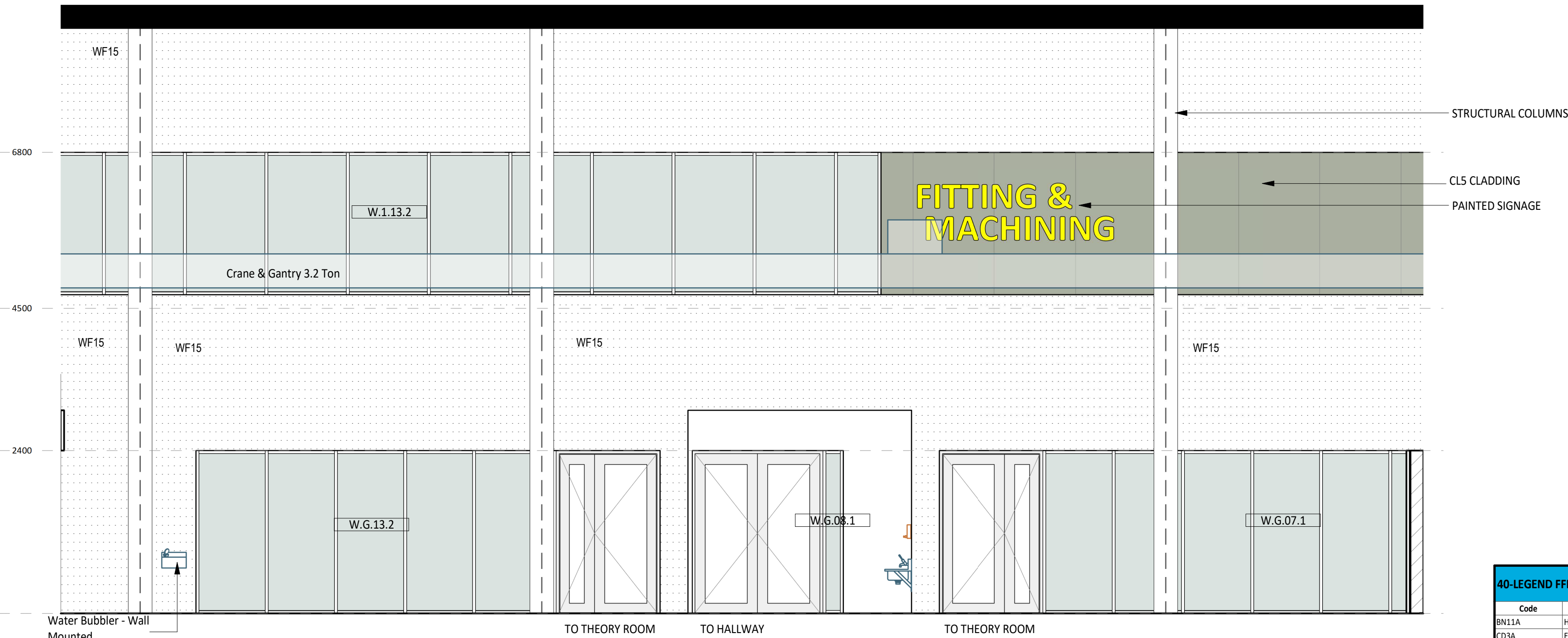
2 60-011 ELEVATION DETAIL 1 : 50
